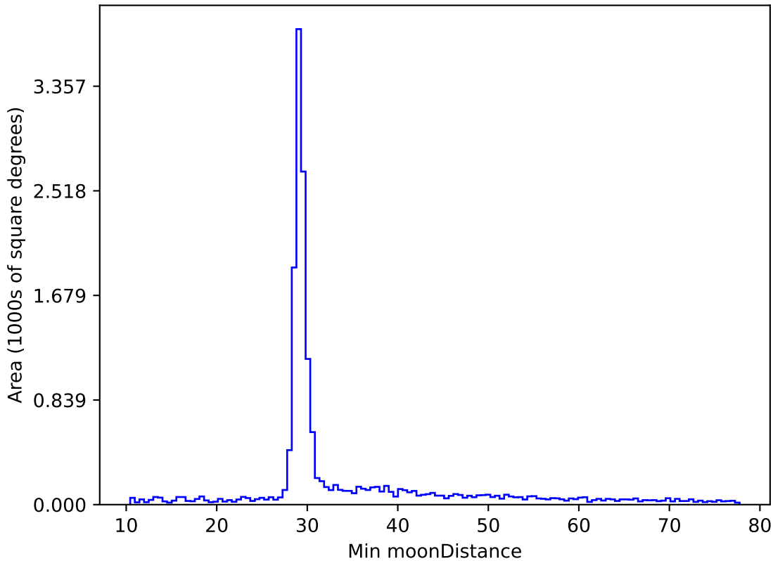
too_elab_r128_d2_gz_v3.4_10yrs WFD all bands: Min moonDistance
