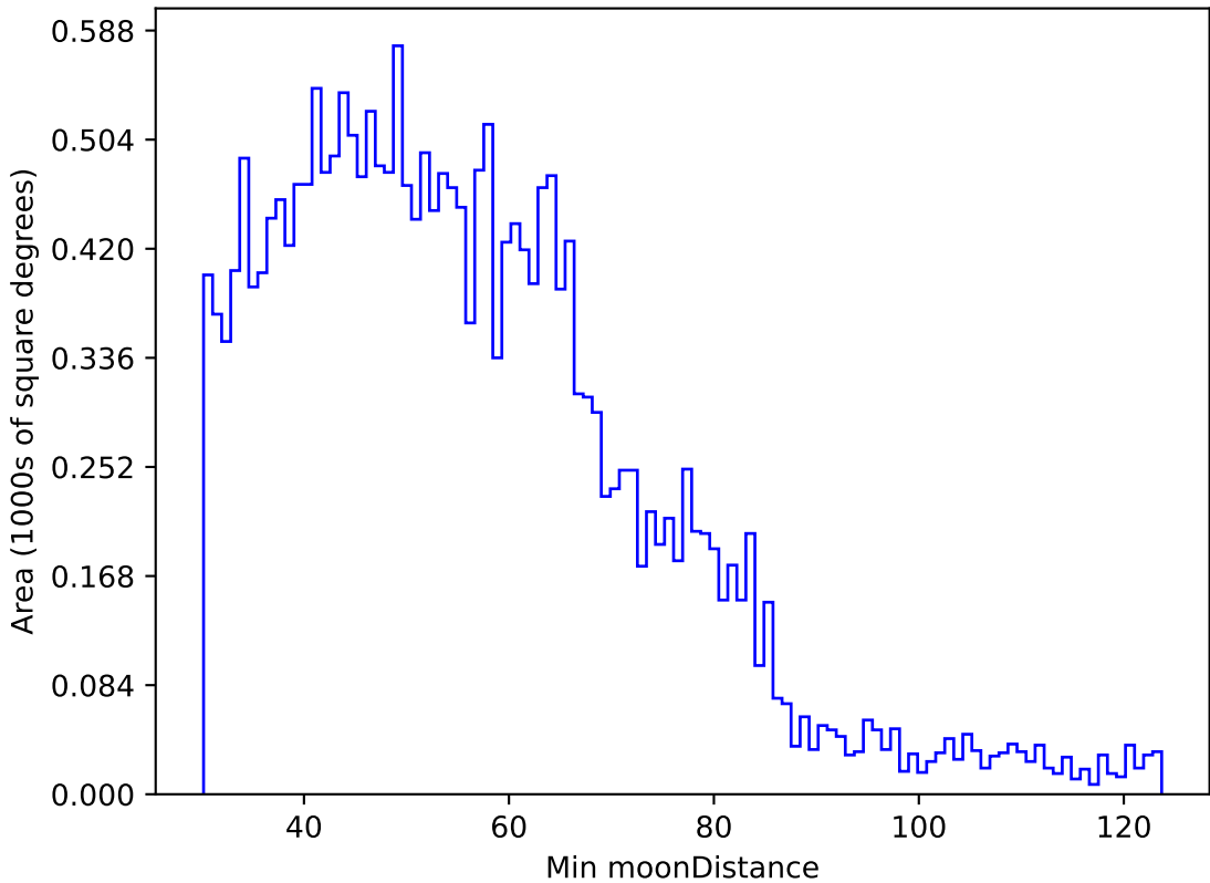
too_elab_r128_d2_gz_v3.4_10yrs All sky u band: Min moonDistance
