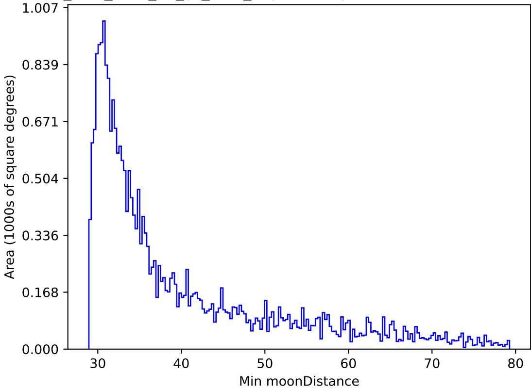
too_elab_r128_d2_gz_v3.4_10yrs All sky r band: Min moonDistance
