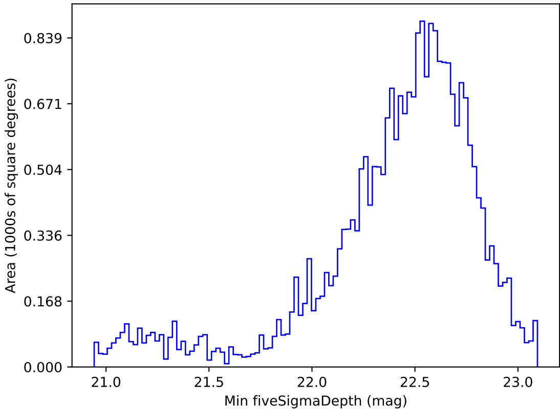
too_elab_r128_d2_gz_v3.4_10yrs Yr 1 z band: Min fiveSigmaDepth
