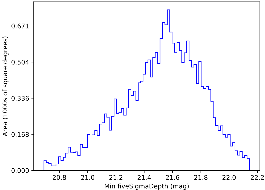
too_elab_r128_d2_gz_v3.4_10yrs Yr 1 y band: Min fiveSigmaDepth
