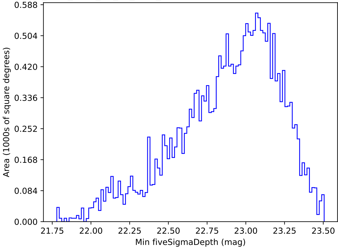
too_elab_r128_d2_gz_v3.4_10yrs Yr 1 u band: Min fiveSigmaDepth
