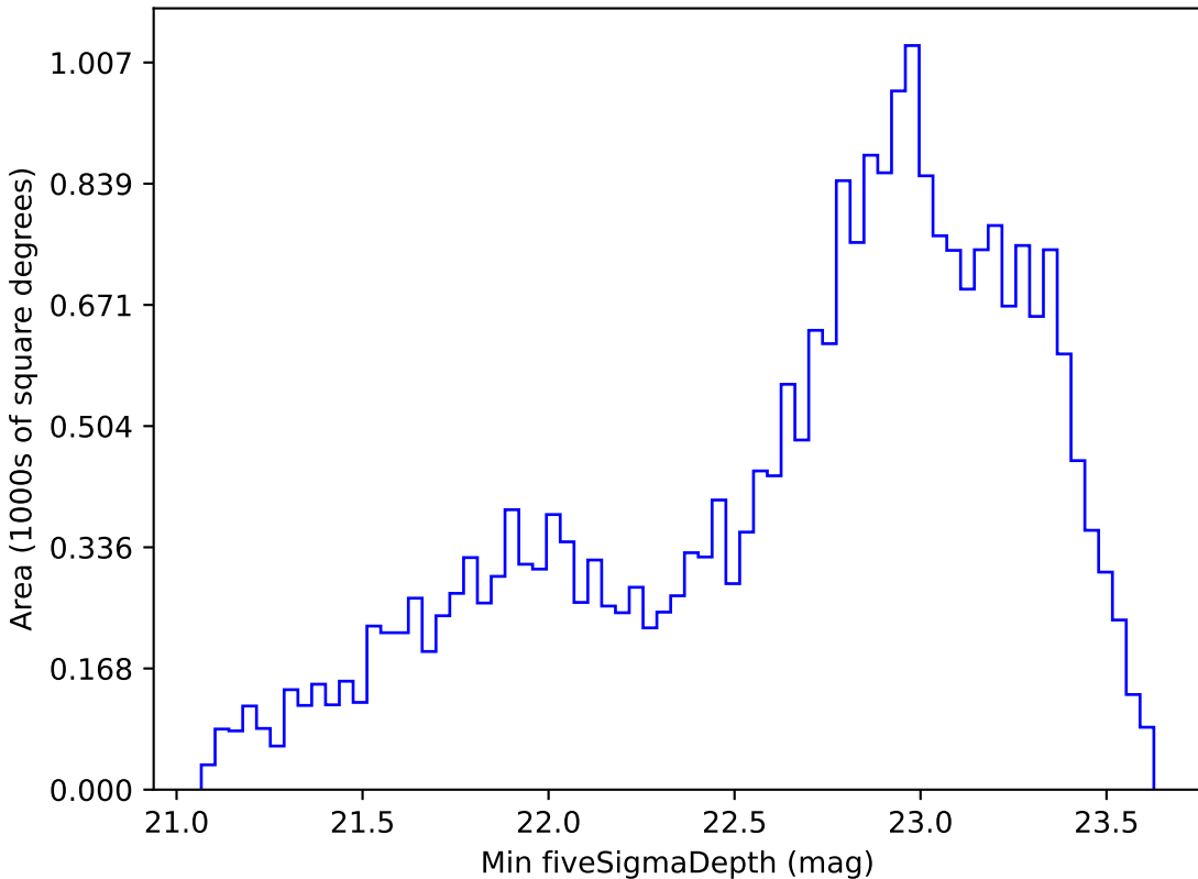
too_elab_r128_d2_gz_v3.4_10yrs Yr 1 i band: Min fiveSigmaDepth
