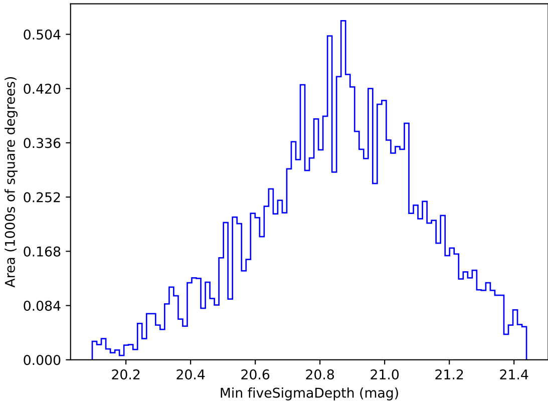
too_elab_r128_d2_gz_v3.4_10yrs WFD y band: Min fiveSigmaDepth
