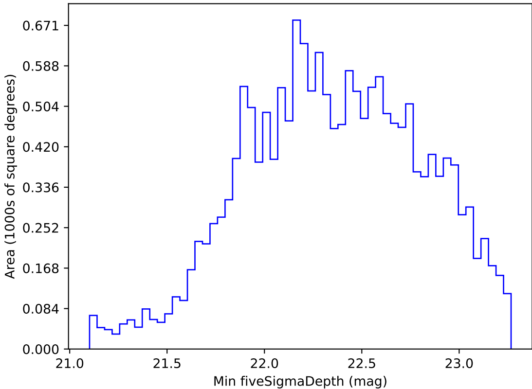
too_elab_r128_d2_gz_v3.4_10yrs WFD r band: Min fiveSigmaDepth
