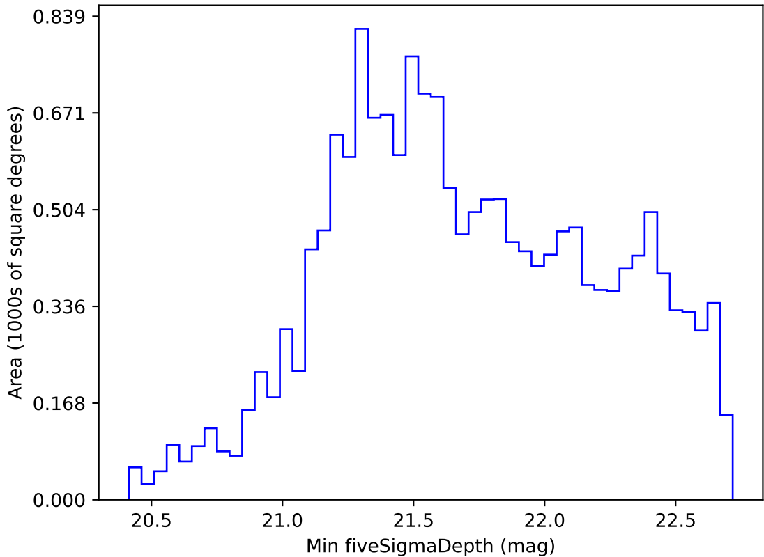
too_elab_r128_d2_gz_v3.4_10yrs WFD i band: Min fiveSigmaDepth
