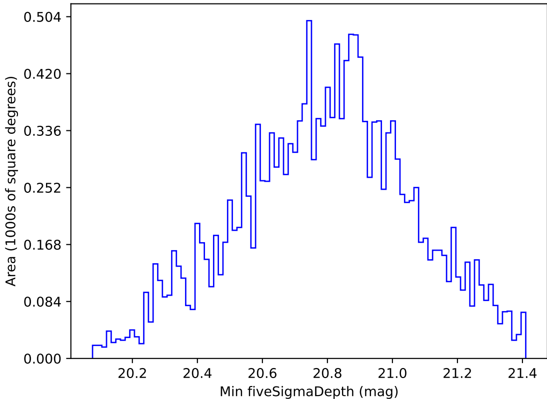
too_elab_r128_d2_gz_v3.4_10yrs WFD all bands: Min fiveSigmaDepth
