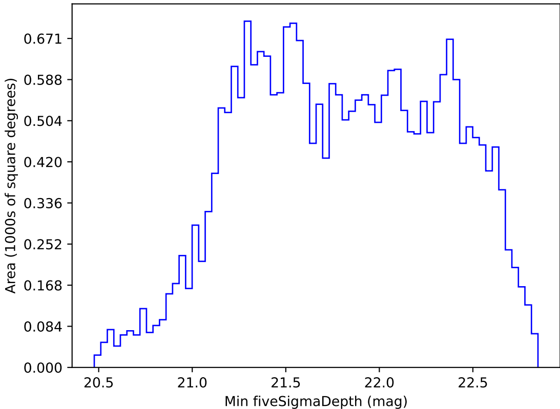
too_elab_r128_d2_gz_v3.4_10yrs All sky i band: Min fiveSigmaDepth
