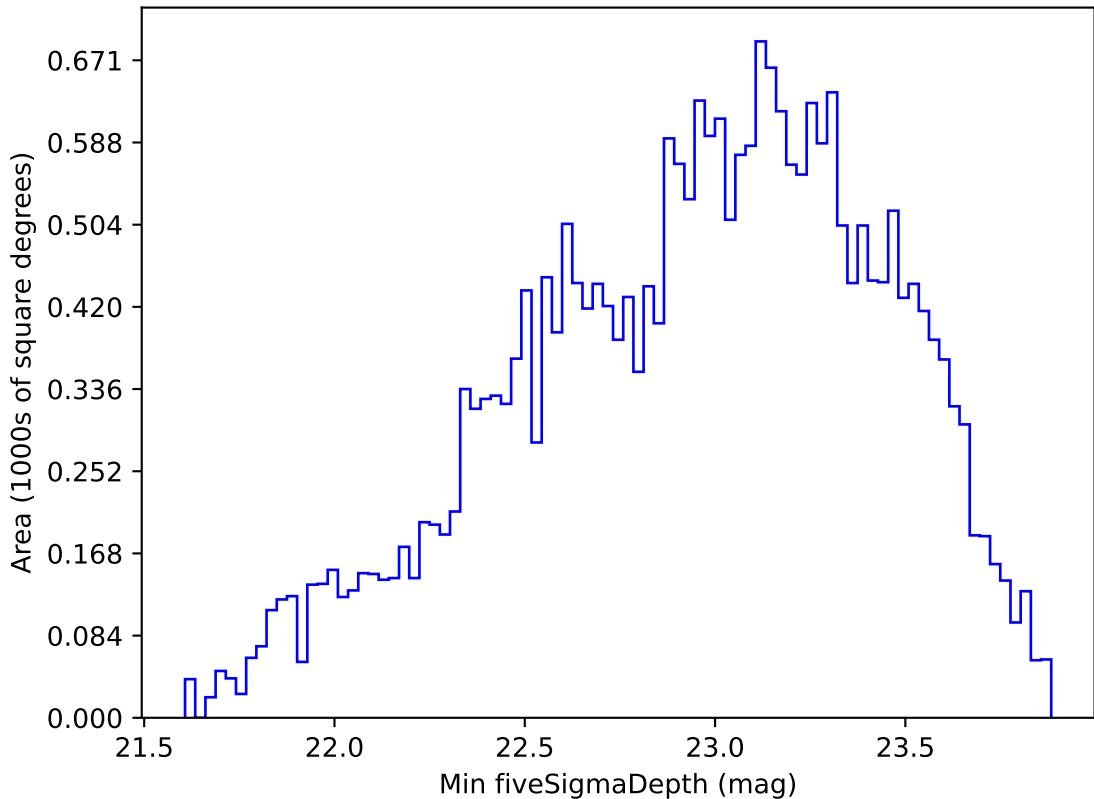
too_elab_r128_d2_gz_v3.4_10yrs All sky g band: Min fiveSigmaDepth
