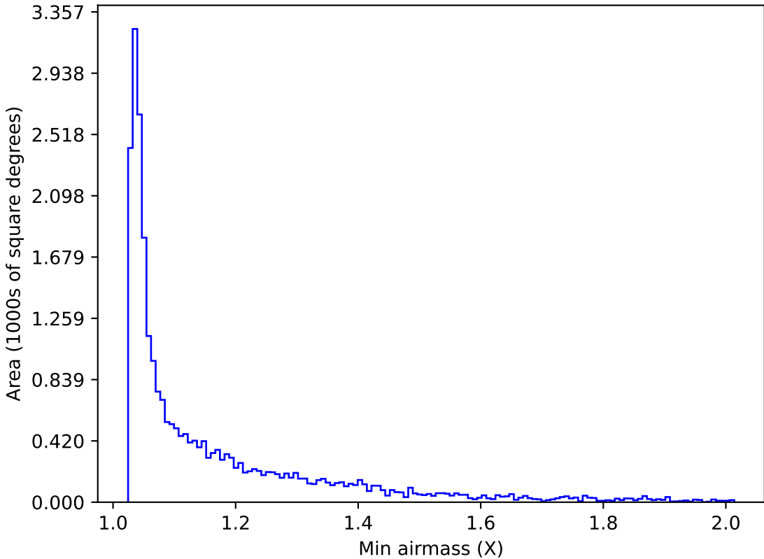
too_elab_r128_d2_gz_v3.4_10yrs Yr 1 i band: Min airmass
