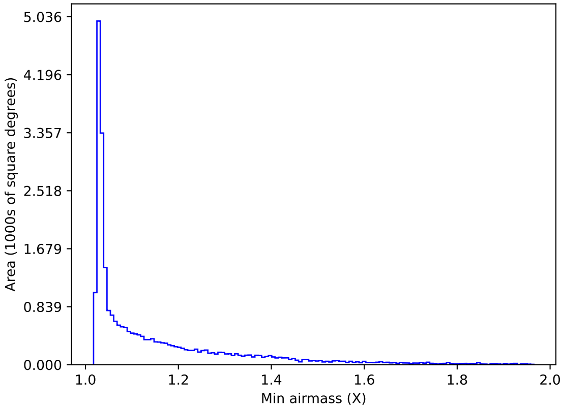
too_elab_r128_d2_gz_v3.4_10yrs Yr 1 all bands: Min airmass
