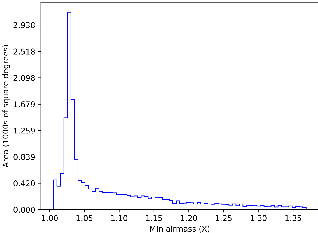
too_elab_r128_d2_gz_v3.4_10yrs WFD z band: Min airmass
