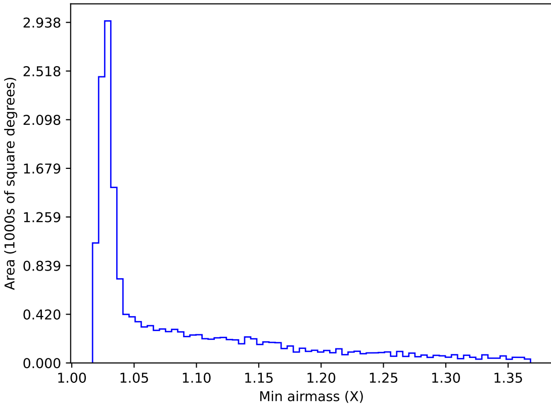
too_elab_r128_d2_gz_v3.4_10yrs WFD r band: Min airmass
