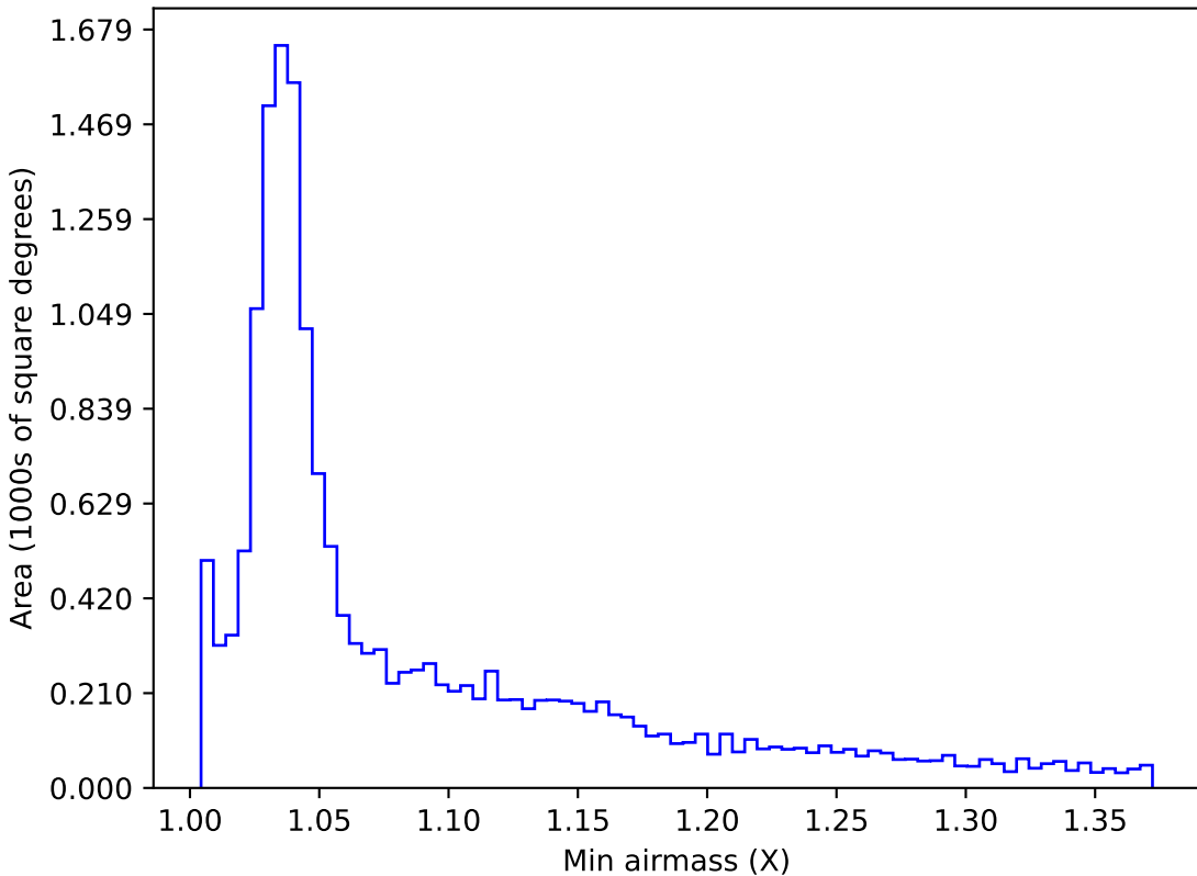
too_elab_r128_d2_gz_v3.4_10yrs WFD g band: Min airmass
