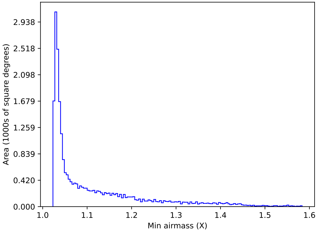
too_elab_r128_d2_gz_v3.4_10yrs All sky y band: Min airmass
