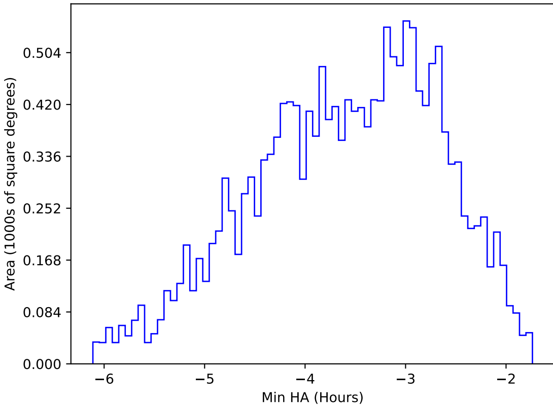
too_elab_r128_d2_gz_v3.4_10yrs WFD y band: Min HA
