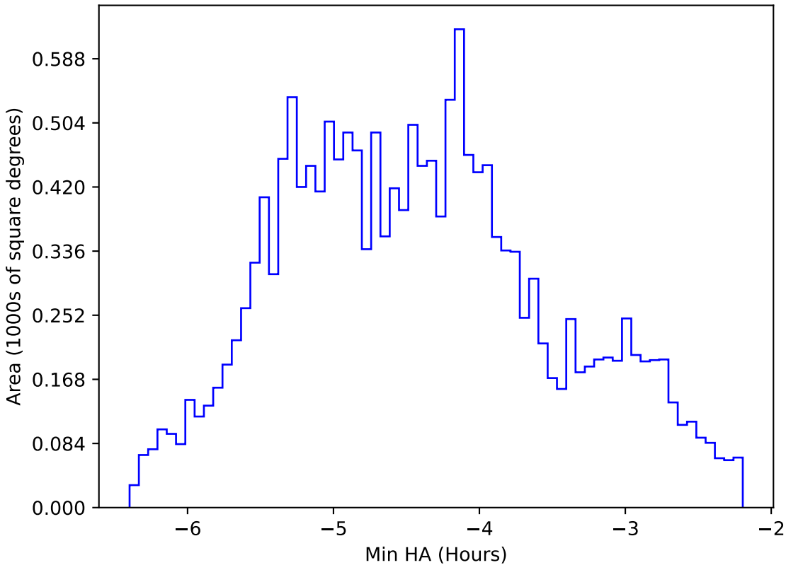
too_elab_r128_d2_gz_v3.4_10yrs WFD r band: Min HA
