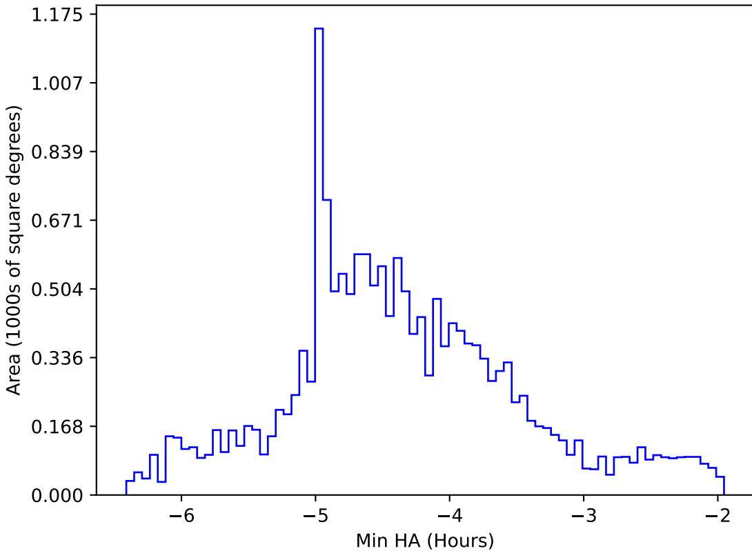
too_elab_r128_d2_gz_v3.4_10yrs WFD g band: Min HA
