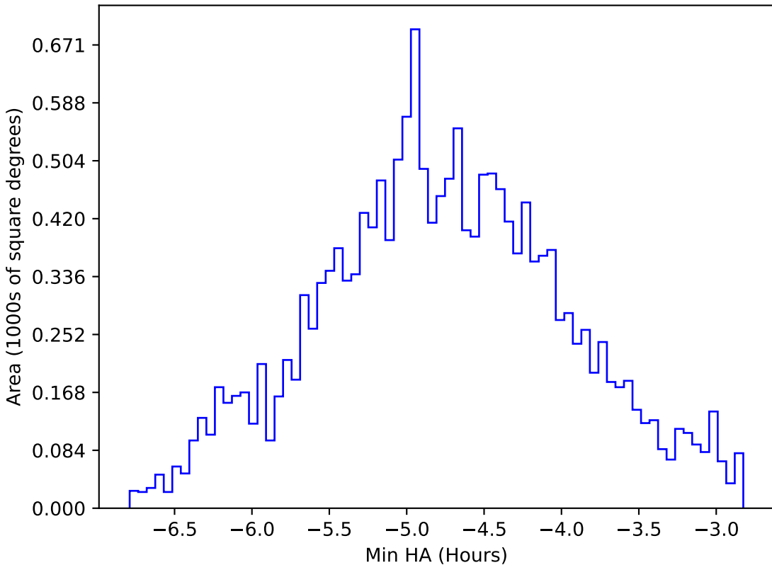
too_elab_r128_d2_gz_v3.4_10yrs WFD all bands: Min HA
