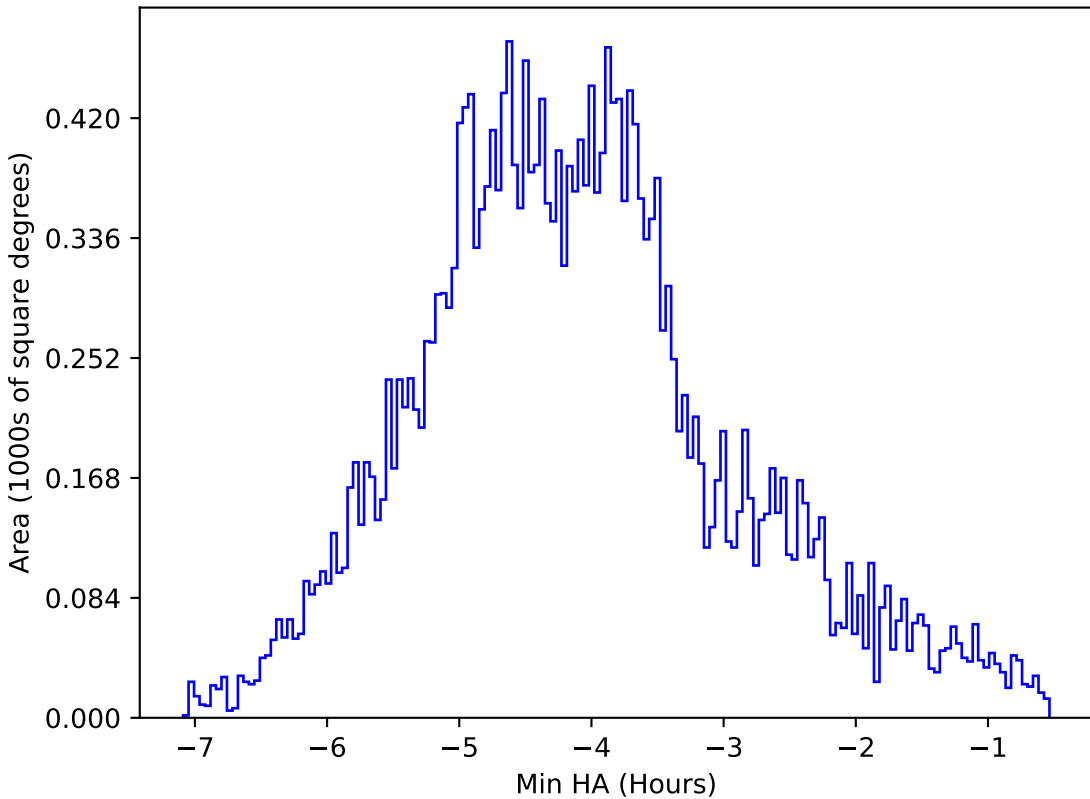
too_elab_r128_d2_gz_v3.4_10yrs All sky z band: Min HA
