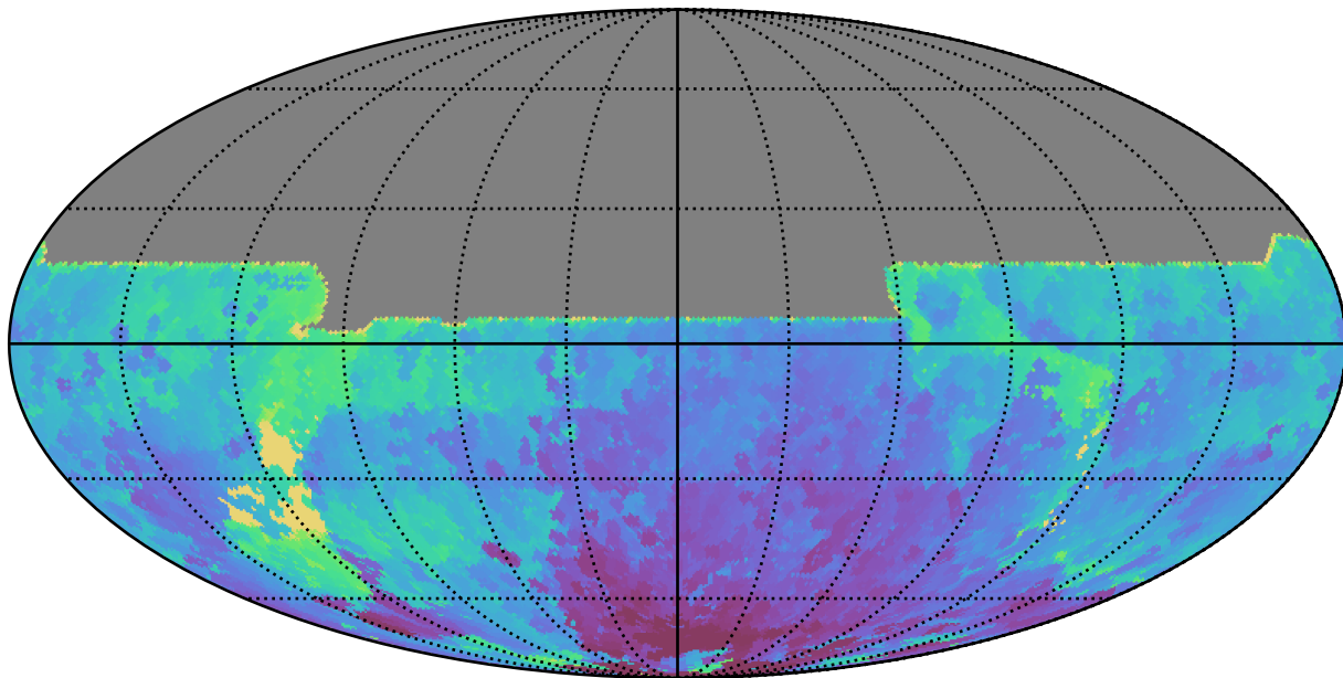
too_elab_r128_d2_gz_v3.4_10yrs All sky y band: Min HA
