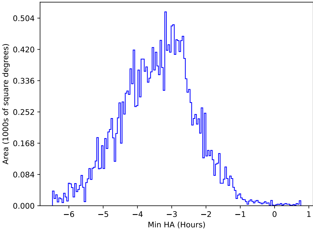
too_elab_r128_d2_gz_v3.4_10yrs All sky y band: Min HA
