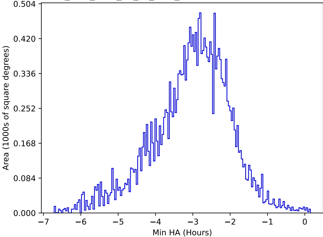
too_elab_r128_d2_gz_v3.4_10yrs All sky u band: Min HA
