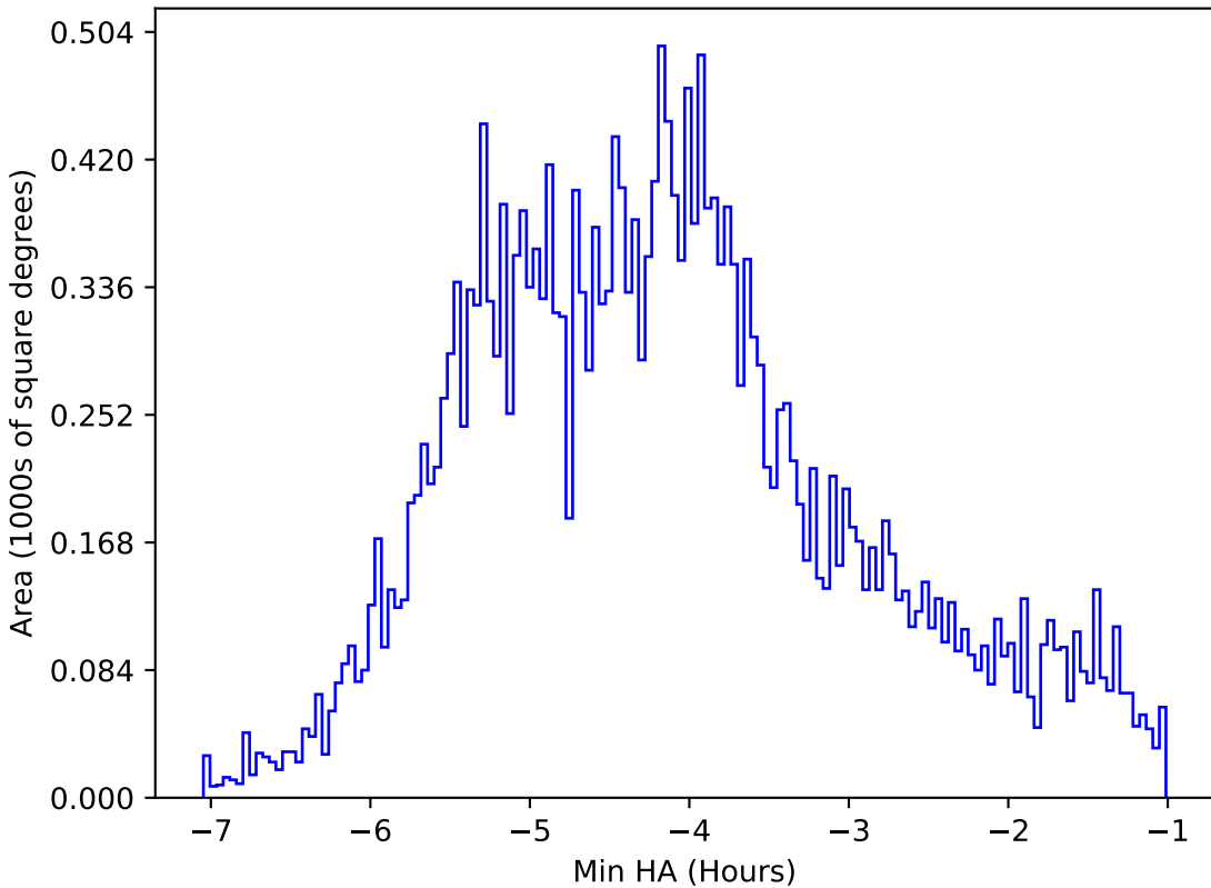
too_elab_r128_d2_gz_v3.4_10yrs All sky r band: Min HA
