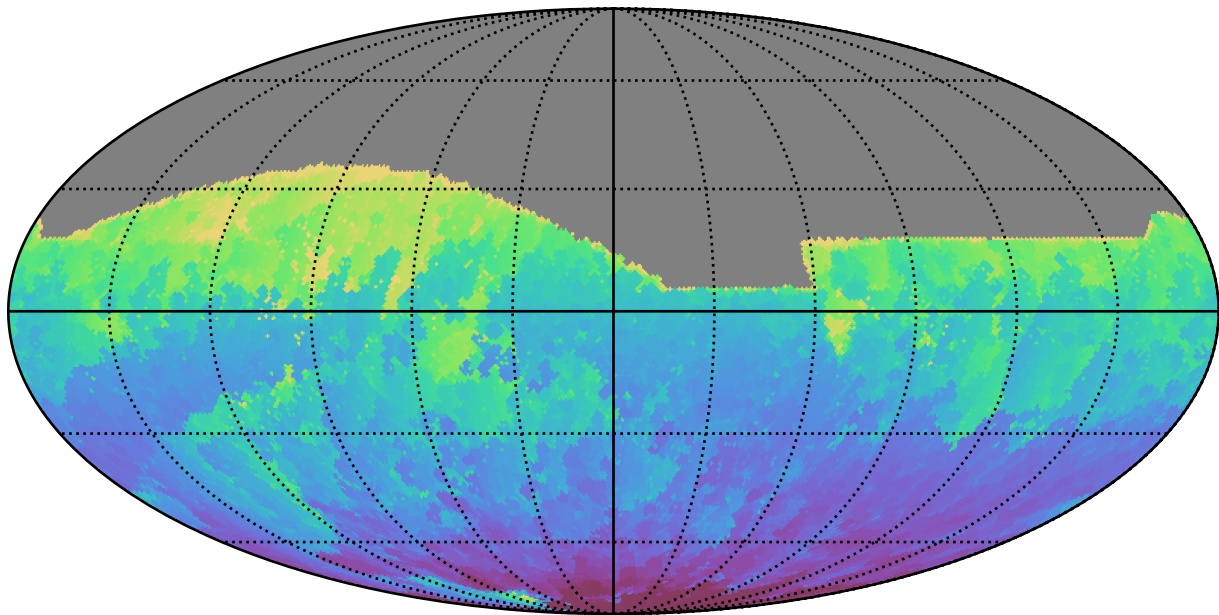
too_elab_r128_d2_gz_v3.4_10yrs All sky i band: Min HA
