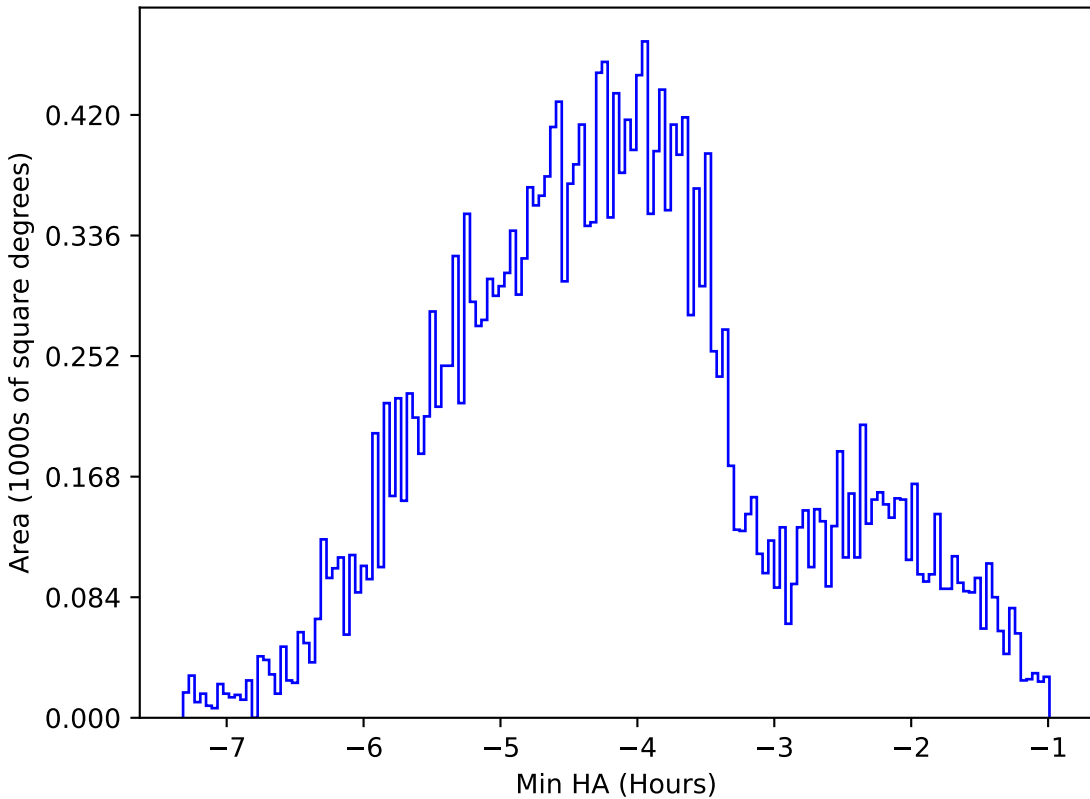
too_elab_r128_d2_gz_v3.4_10yrs All sky i band: Min HA
