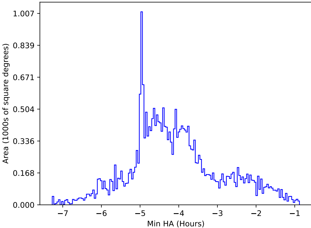
too_elab_r128_d2_gz_v3.4_10yrs All sky g band: Min HA
