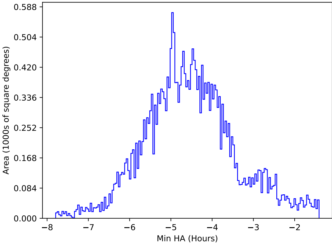
too_elab_r128_d2_gz_v3.4_10yrs All sky all bands: Min HA
