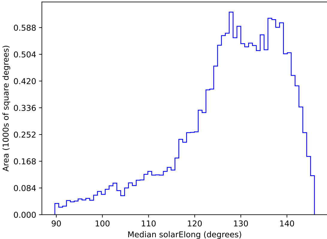
too_elab_r128_d2_gz_v3.4_10yrs WFD z band: Median solarElong
