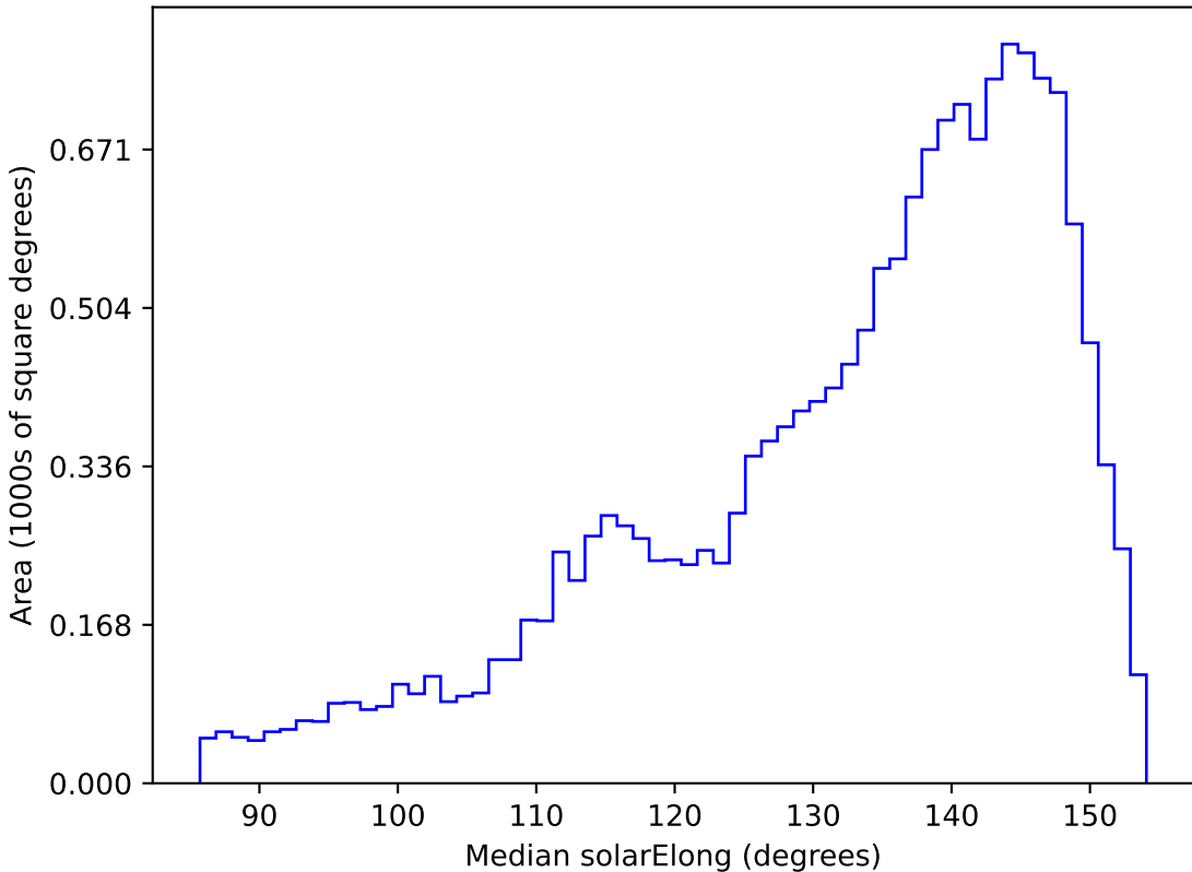
too_elab_r128_d2_gz_v3.4_10yrs WFD u band: Median solarElong
