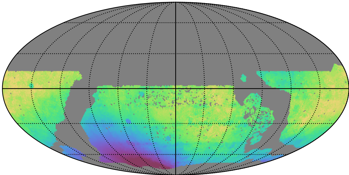
too_elab_r128_d2_gz_v3.4_10yrs WFD r band: Median solarElong
