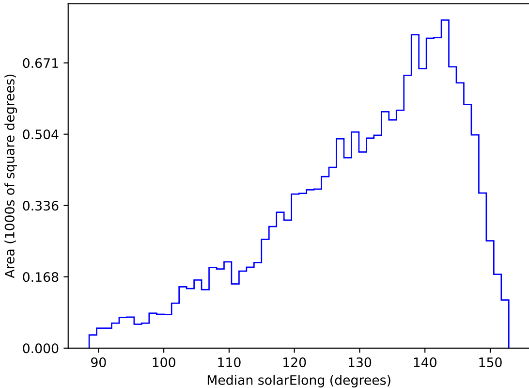
too_elab_r128_d2_gz_v3.4_10yrs WFD g band: Median solarElong
