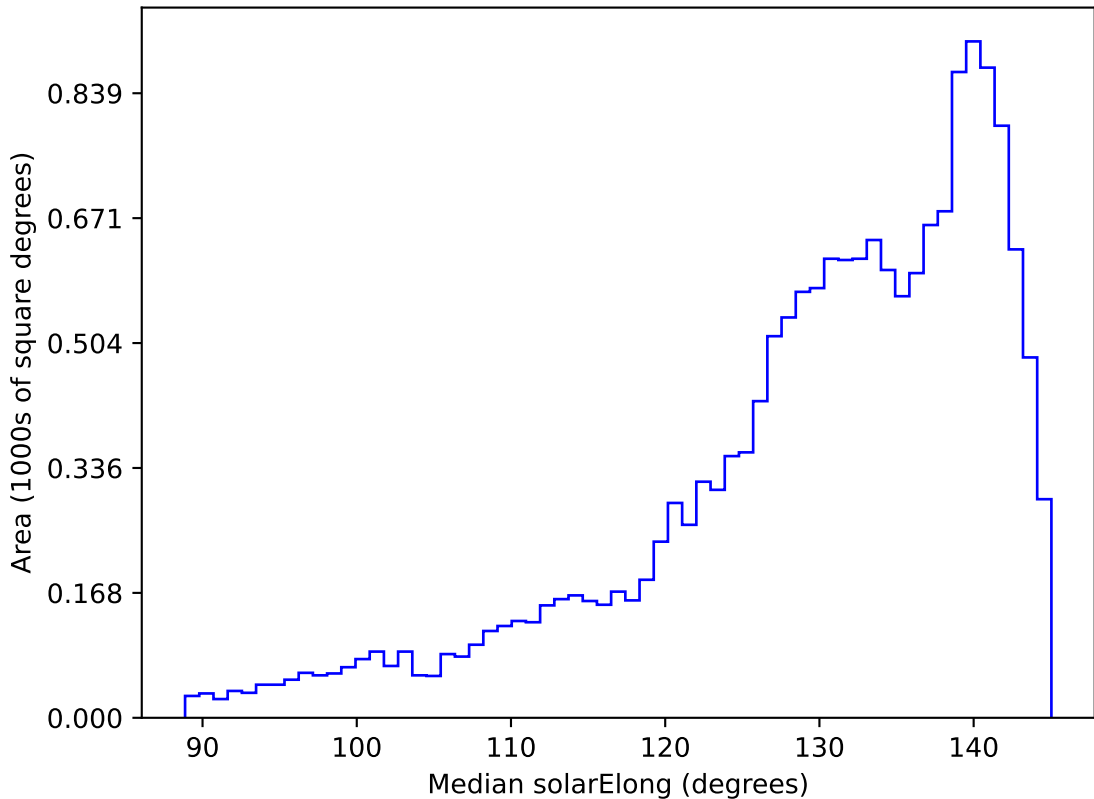
too_elab_r128_d2_gz_v3.4_10yrs WFD all bands: Median solarElong
