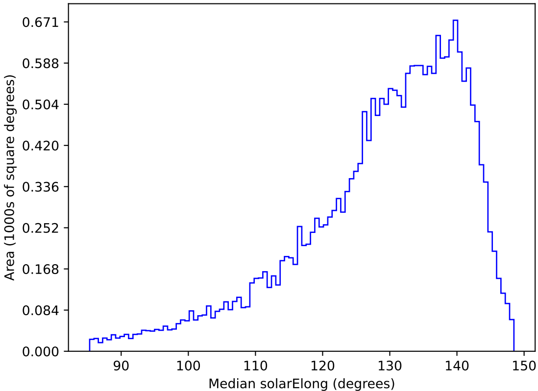
too_elab_r128_d2_gz_v3.4_10yrs All sky y band: Median solarElong
