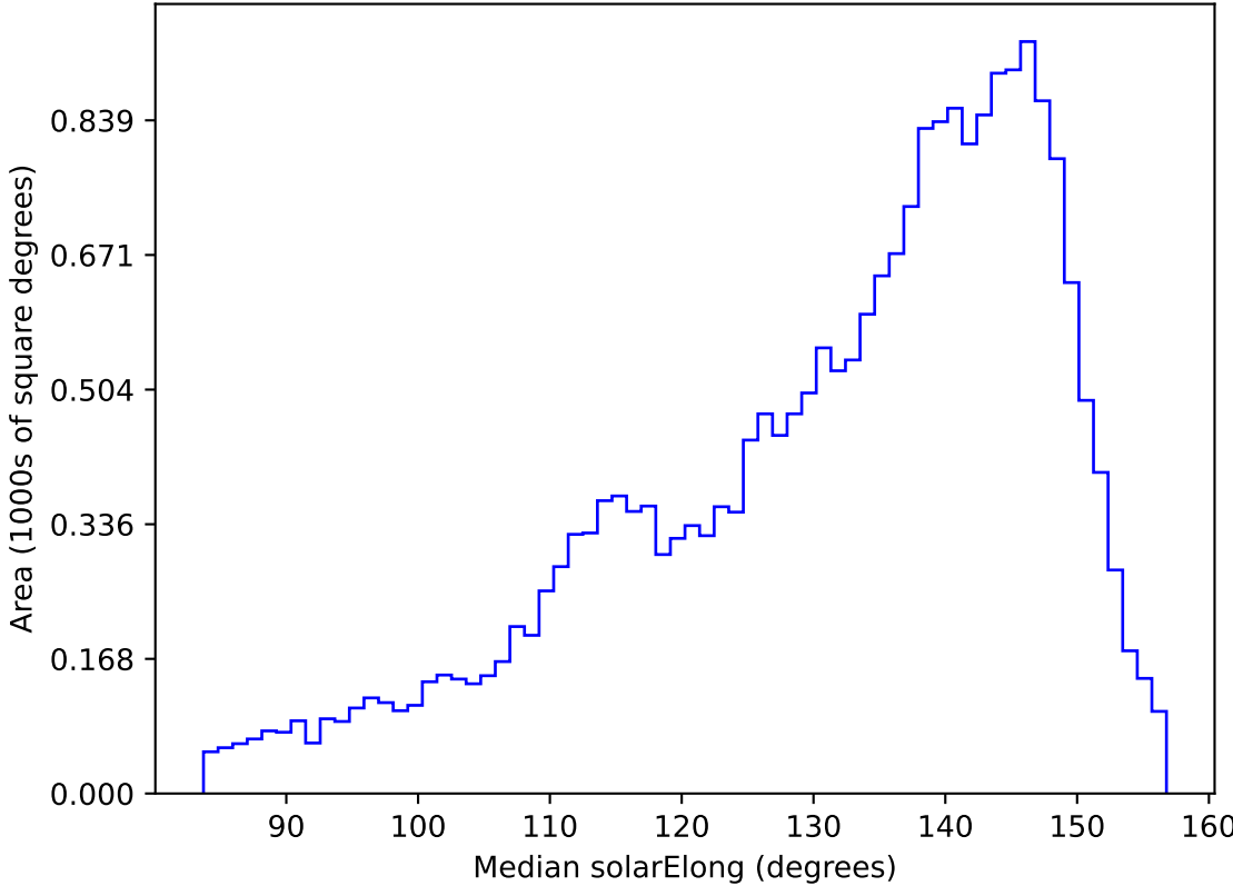
too_elab_r128_d2_gz_v3.4_10yrs All sky u band: Median solarElong
