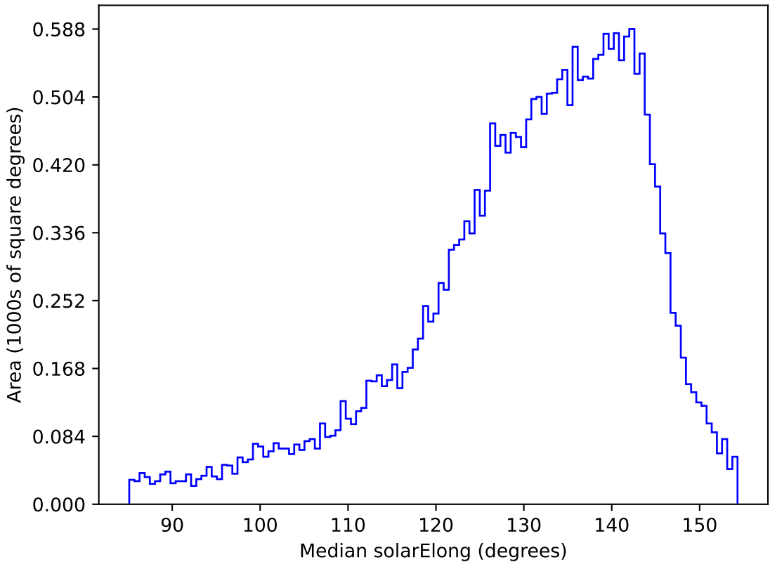
too_elab_r128_d2_gz_v3.4_10yrs All sky r band: Median solarElong
