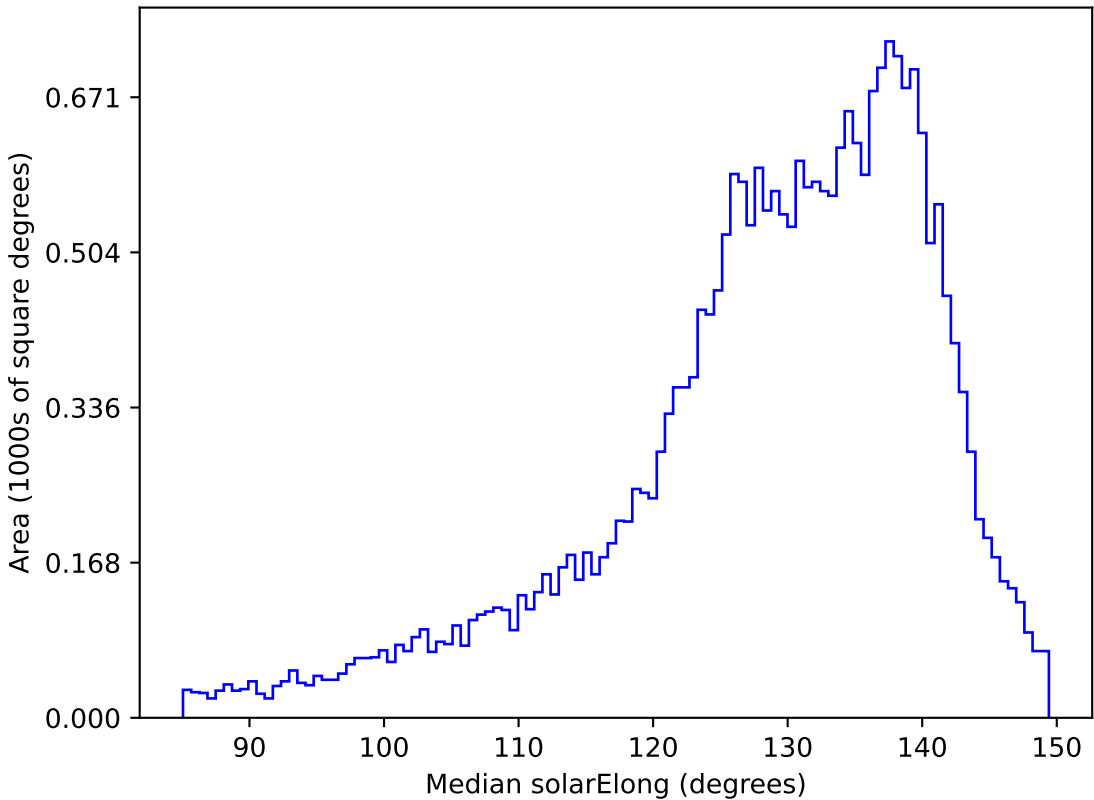
too_elab_r128_d2_gz_v3.4_10yrs All sky i band: Median solarElong
