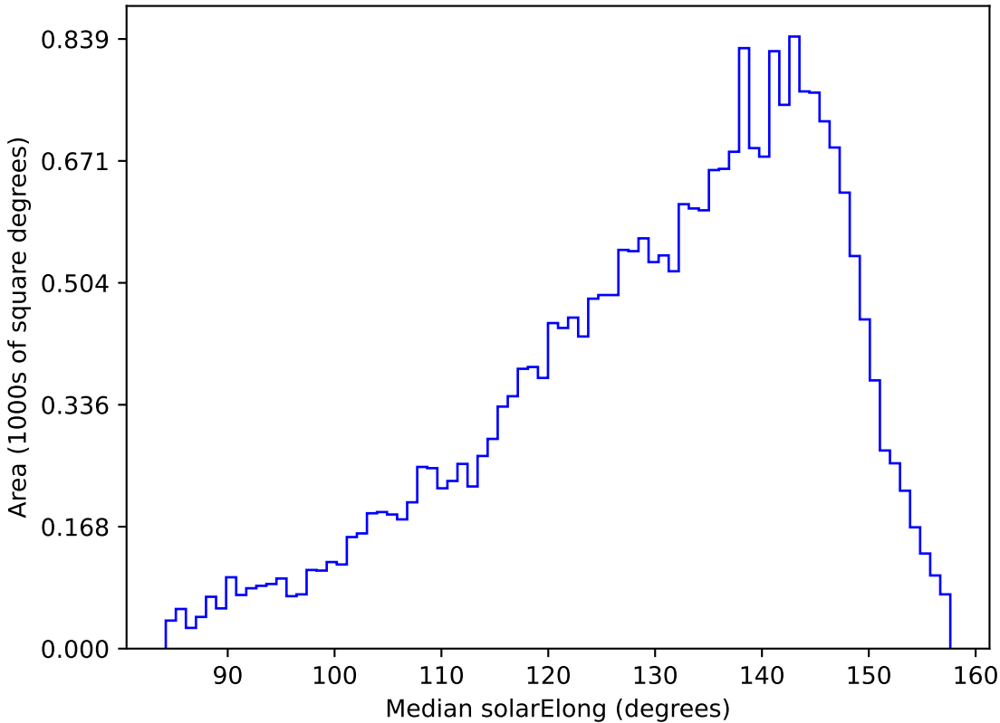
too_elab_r128_d2_gz_v3.4_10yrs All sky g band: Median solarElong
