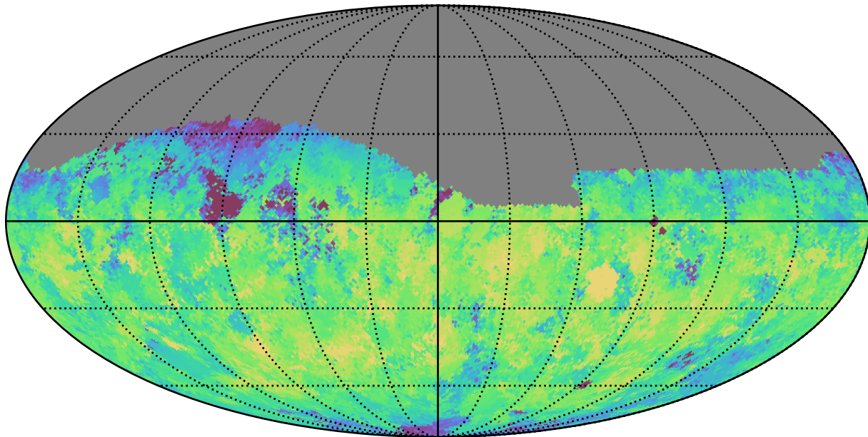
too_elab_r128_d2_gz_v3.4_10yrs Yr 1 z band: Median skyBrightness
