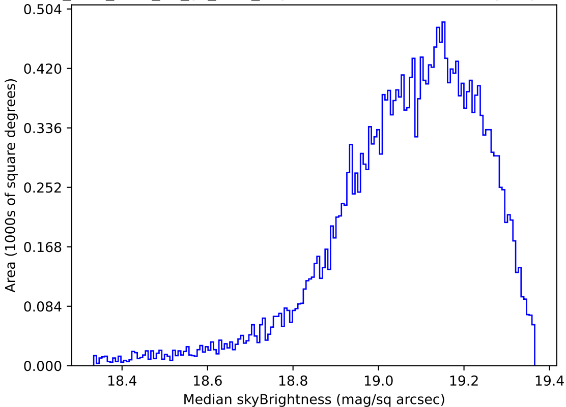
too_elab_r128_d2_gz_v3.4_10yrs Yr 1 z band: Median skyBrightness
