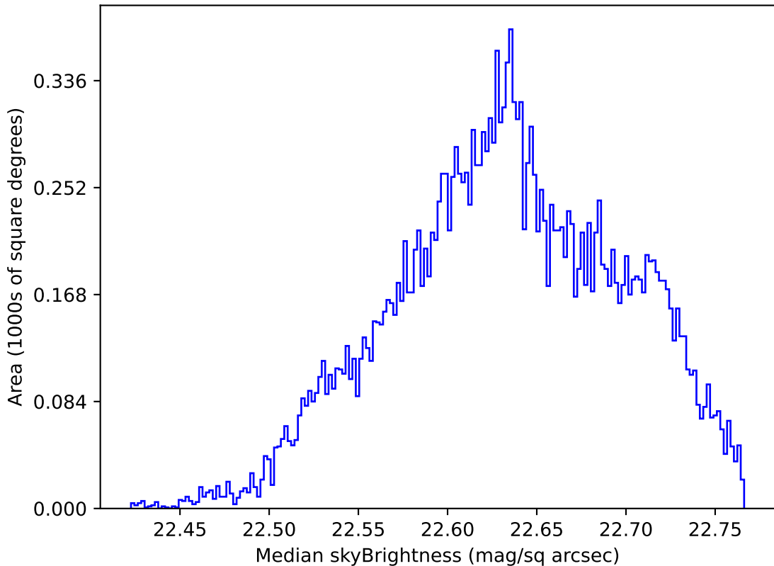
too_elab_r128_d2_gz_v3.4_10yrs Yr 1 u band: Median skyBrightness
