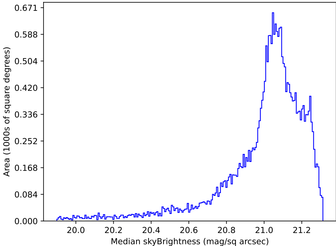
too_elab_r128_d2_gz_v3.4_10yrs Yr 1 r band: Median skyBrightness
