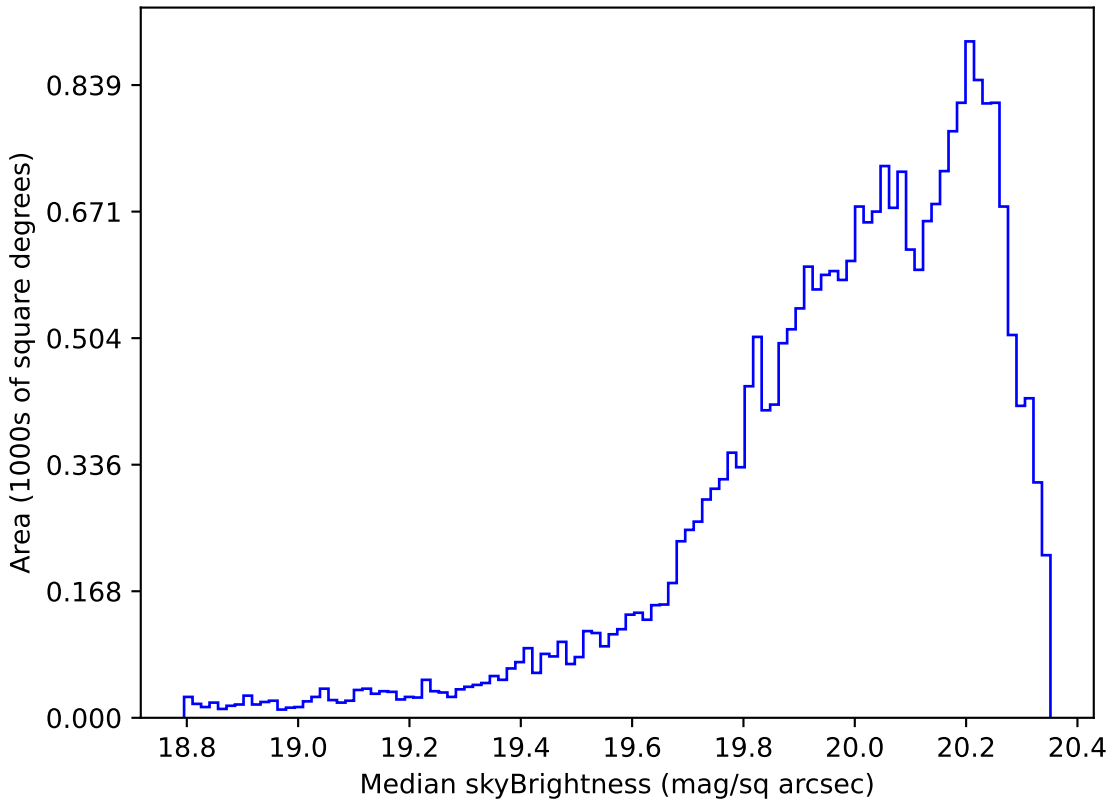
too_elab_r128_d2_gz_v3.4_10yrs Yr 1 i band: Median skyBrightness
