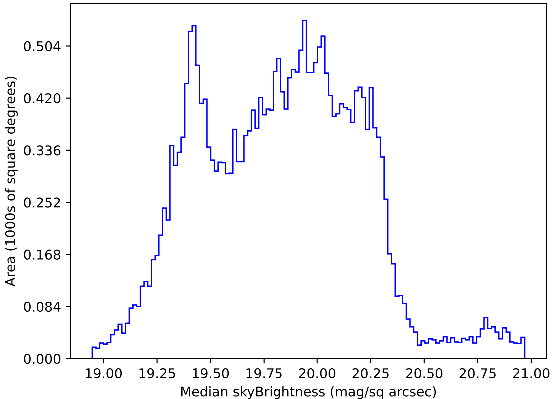
too_elab_r128_d2_gz_v3.4_10yrs Yr 1 all bands: Median skyBrightness
