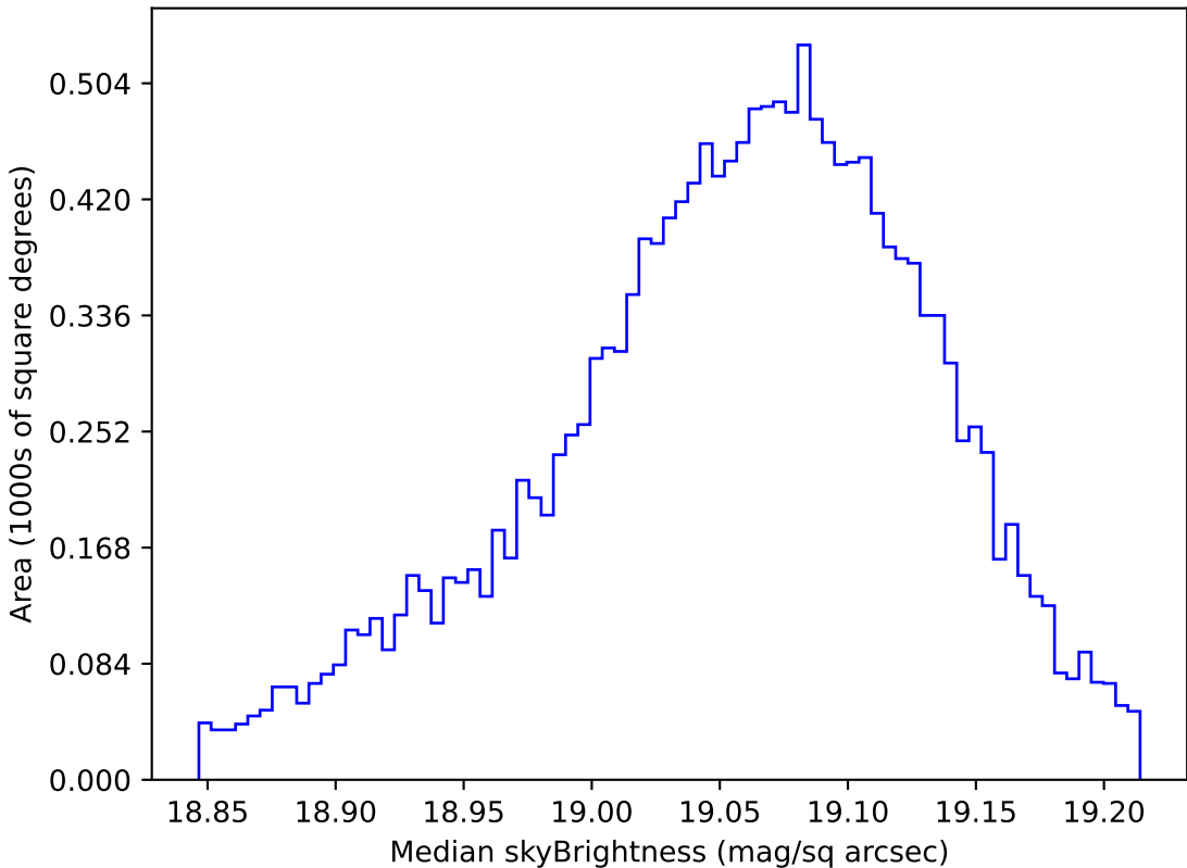
too_elab_r128_d2_gz_v3.4_10yrs WFD z band: Median skyBrightness
