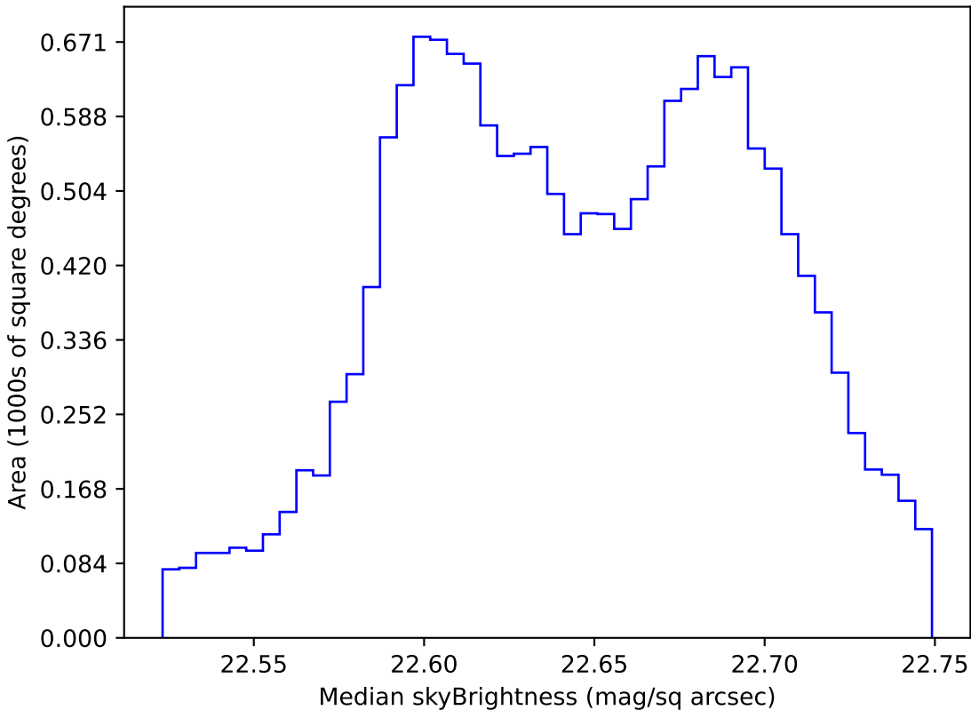
too_elab_r128_d2_gz_v3.4_10yrs WFD u band: Median skyBrightness
